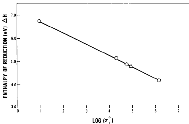
Fig. 6. Correlation between oxide reduction ( \Delta\bar{H} ) and ionic conductivity ( \sigma_i^0 ) for: \circ , (\text{ZrO}_2)_{0.85}(\text{CaO})_{0.15} ; \square , (\text{CeO}_2)_{0.82}(\text{La}_2\text{O}_3)_{0.18} ; \diamond , (\text{CeO}_2)_{0.95}(\text{CaO})_{0.05} ; \triangle , (\text{CeO}_2)_{0.95}(\text{Y}_2\text{O}_3)_{0.05} ; \circ , (\text{CeO}_2)_{0.82}(\text{Gd}_2\text{O}_3)_{0.18} .
