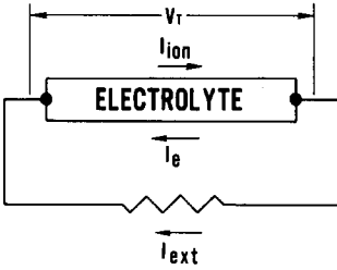
Fig. 1. Equivalent circuit for mixed-conducting solid electrolyte.
